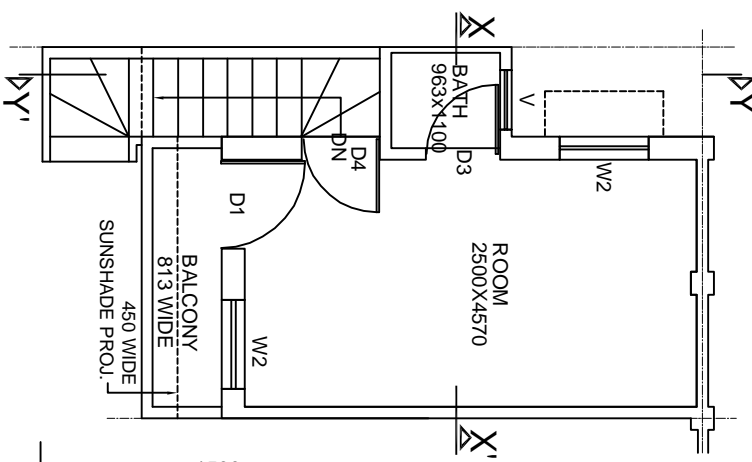
FIRST FLOOR PLAN SCALE -1:100
