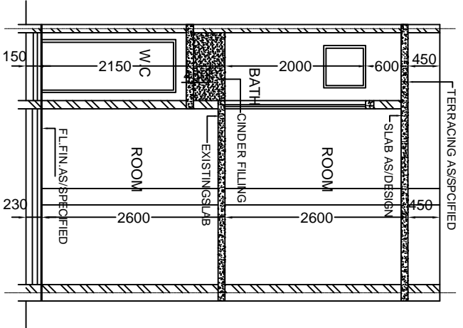
SECTION AT X-X' SCALE -1:100
