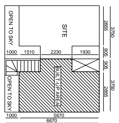
SITE PLAN SCALE -1:50
