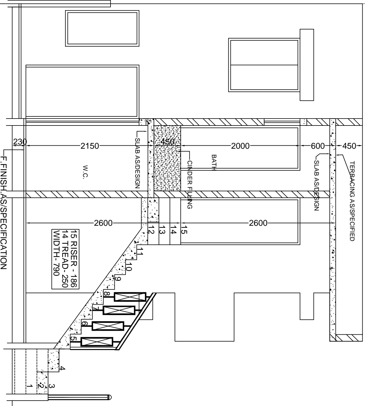
SECTION AT Y-Y' SCALE -1:50
