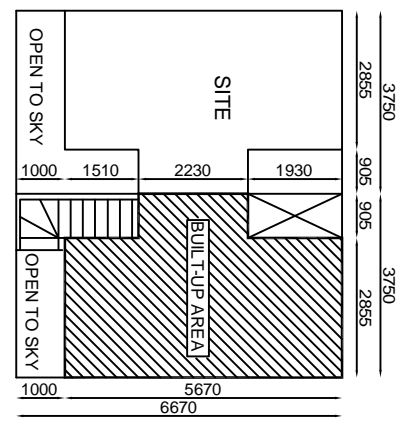
SITE PLAN SCALE -1:50
