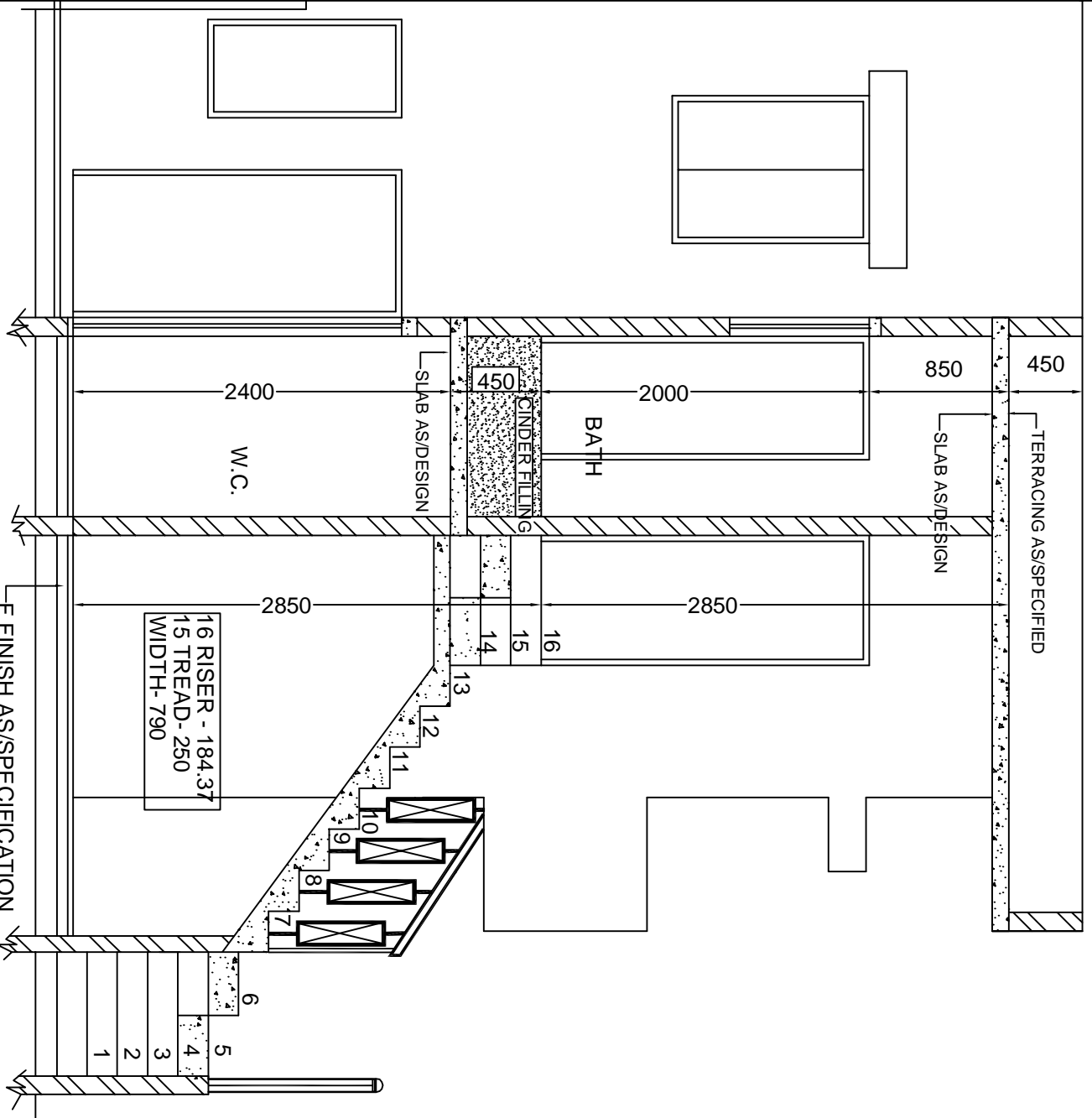
SECTION AT Y-Y' SCALE -1:50
