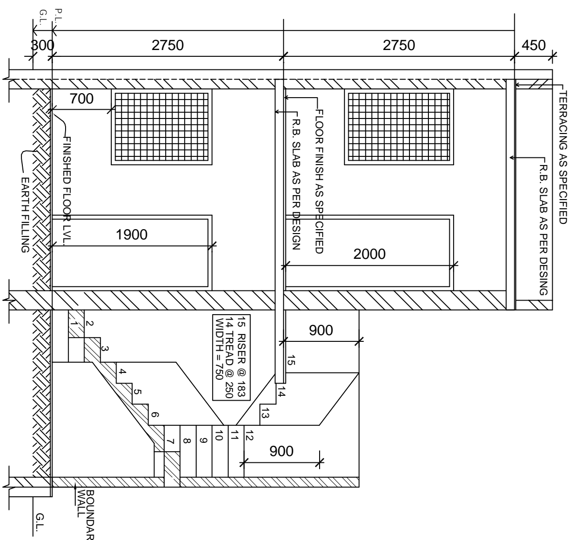
SECTION AT X-X' SCALE - 1:50
