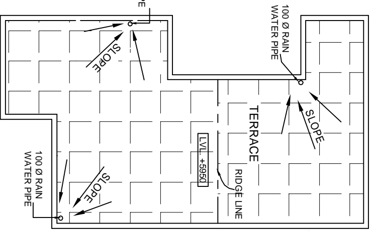
TERRACE PLAN SCALE - 1:100
