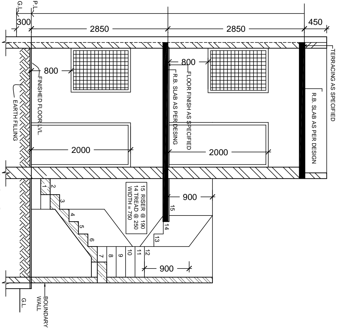
SECTION AT X-X' SCALE - 1:50
