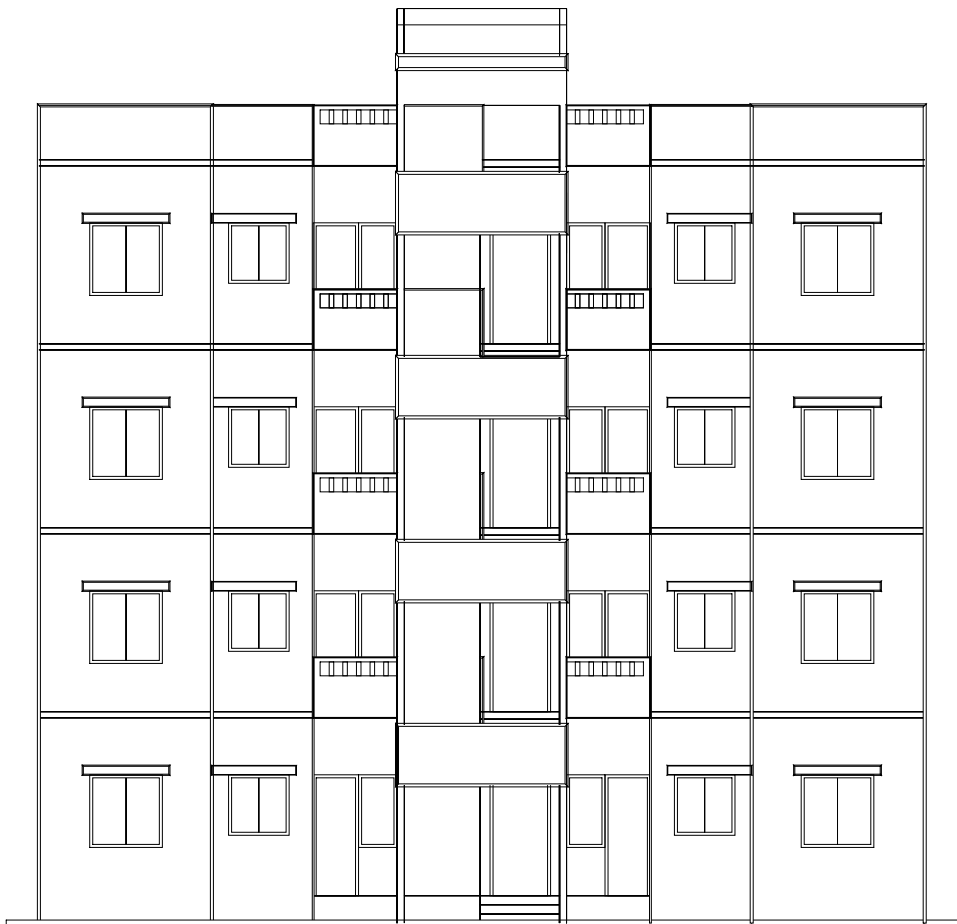
TYPICAL ROW HOUSING FRONT ELEVATION OF CLUSTERS
