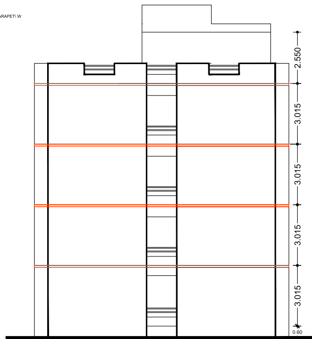
SIDE ELEVATION
