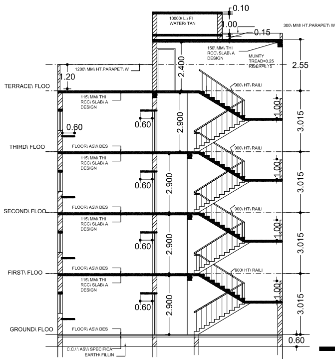
SECTION ELEVATION
